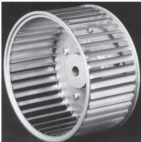
SINGLE WIDTH LEFT HAND MULTIVANE IMPELLER WITH FLANGED HUB (CLOCKWISE)
