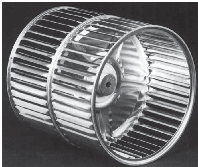
DOUBLE WIDTH RIGHT HAND MULTIVANE IMPELLER WITH CLINCH TYPE HUB (ANTICLOCKWISE)
